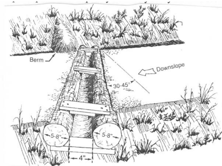
Figure 5-10. Open-top log culvert.
