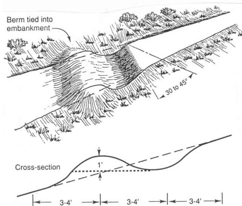
Figure 5-12. Water bar.
