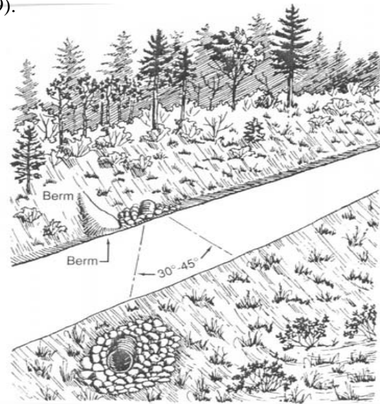
Figure 5-9. Cross-drain culvert.
