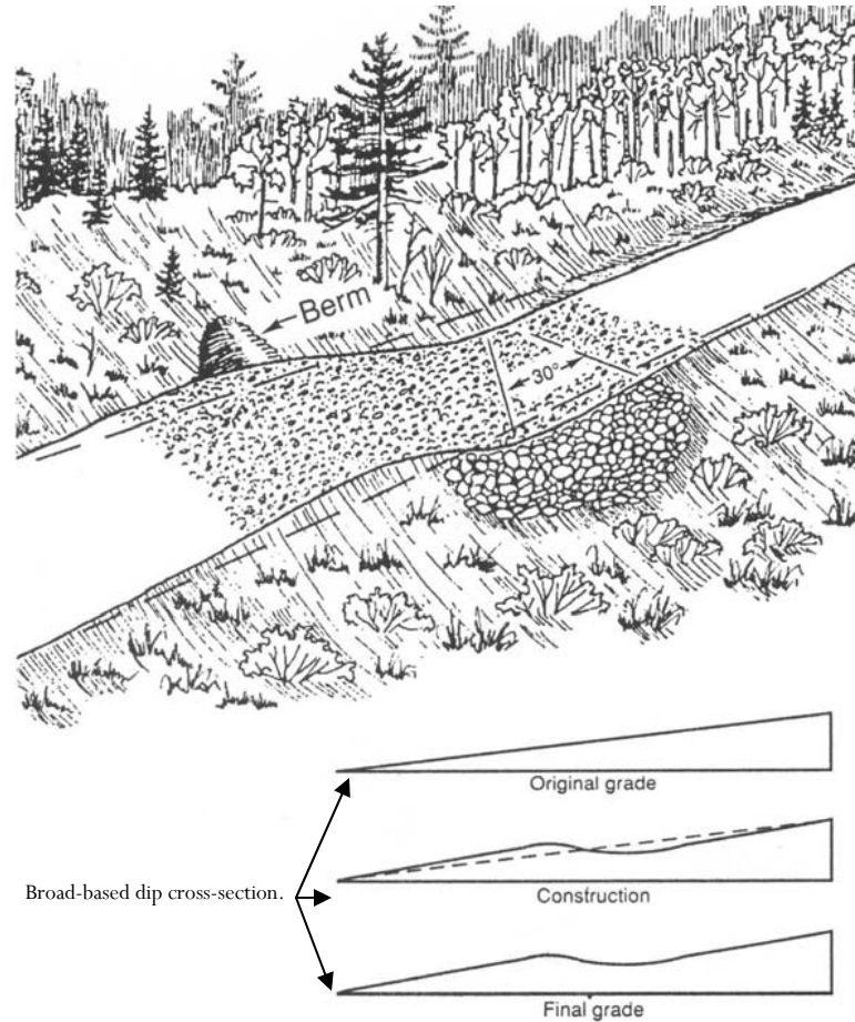
Figure 5-11. Broad-based dip.
