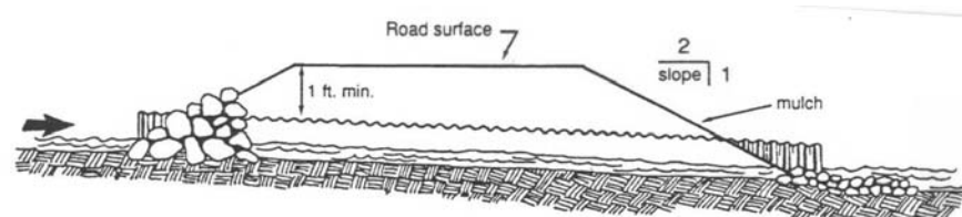
Figure 5-5. Install culverts so there is no change in the stream bottom elevation.
