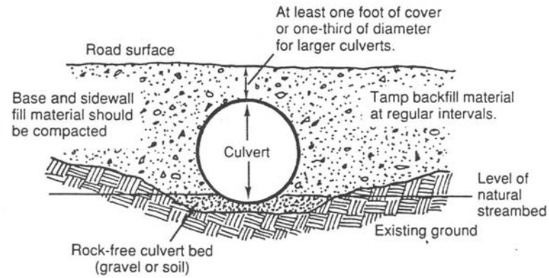
Figure 5-6. Installation of culverts. (Adapted from Montana Department of State Lands, 1992.)
