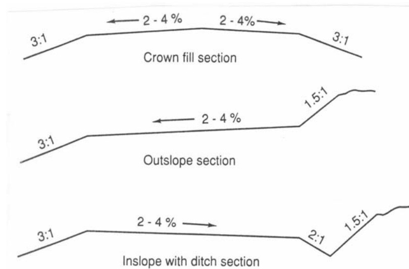
Figure 5-8. Typical road designs for drainage and stability.
